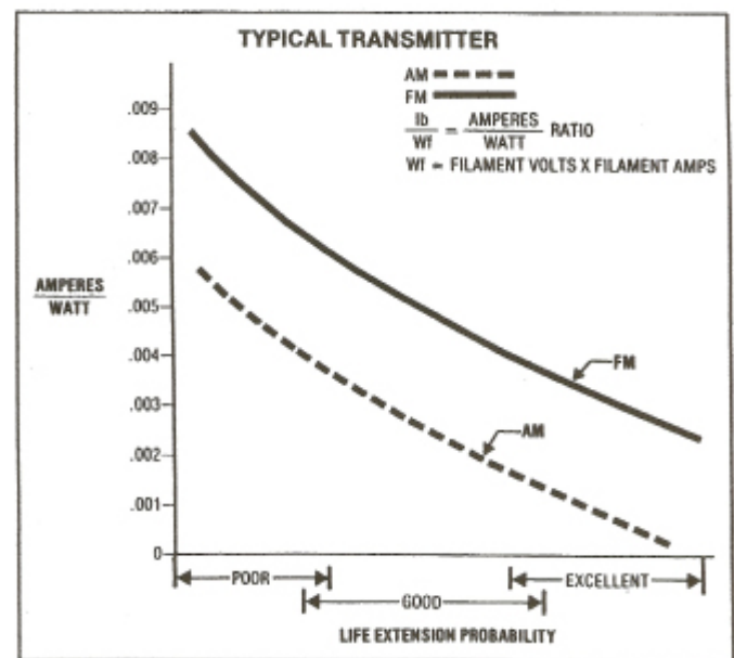
Figure 1. The probability of extended life service can be determined from this graph. Divide the average anode current in amperes by the product of filament voltage and current. The resulting amperes/watt ratio is projected horizontally to the appropriate curve. The vertical projection to the X-axis indicates the life extension probability.
